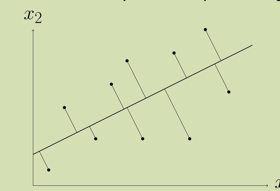
Figure 4: Orthogonal regression
